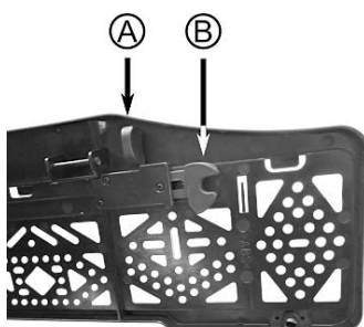
Figure 10: Locking mechanism
