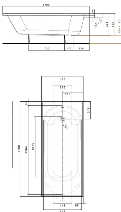
Abmessungen in mm
