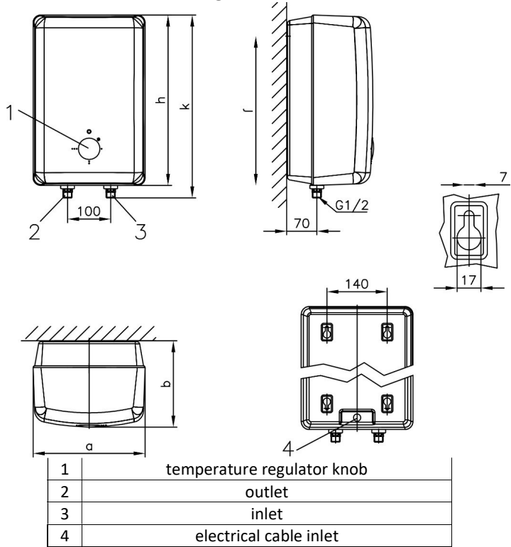
Mounting dimensions (mm)
