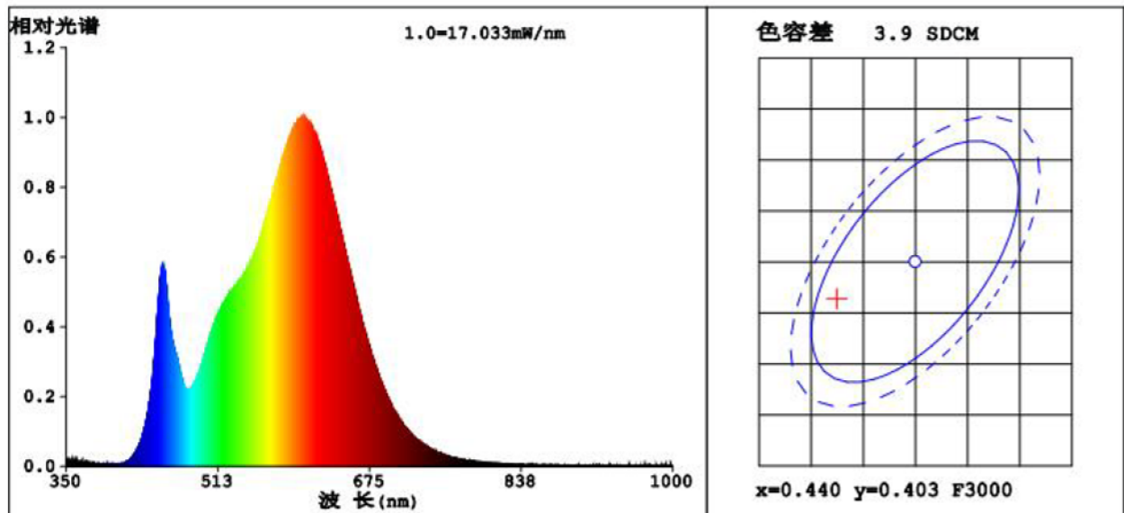
Attachment No. 1: Photometric test record of one lamp at initial measurement
