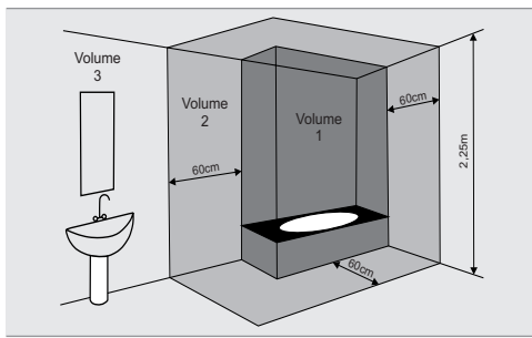
Fig. 1: Safety distances
