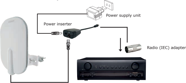
Connection example:
